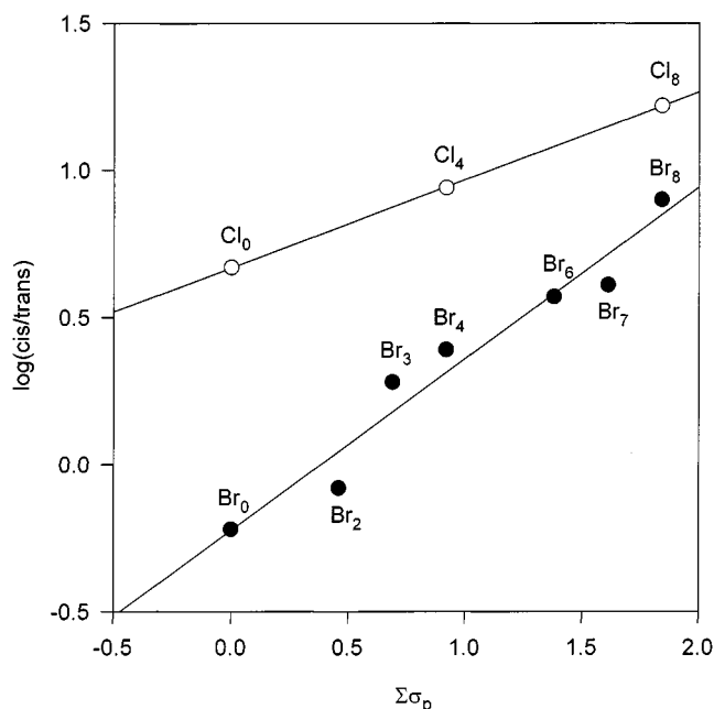
Figure 1. Correlation diagram of the logarithm of the cis/trans epoxides ratio vs. the sum of Hammett's \sigma_p for the epoxidation of cis -stilbene catalysed by a series of progressively \beta -halogenated MnTPPBr (filled circles) and MnTDMPPCl (open circles)
