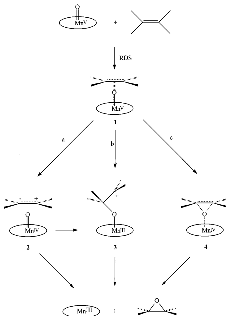
Scheme 1. Unified mechanism for the oxygen transfer from oxo-metalloporphyrins to alkenes [8]
